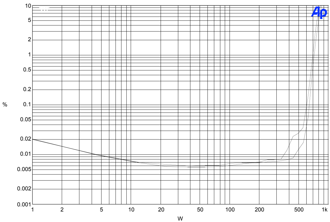
Bel Canto eVo2 bridged (4 ohm load)
